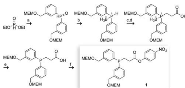
Scheme 2. Synthetic Route to Phosphinoester 1 a
